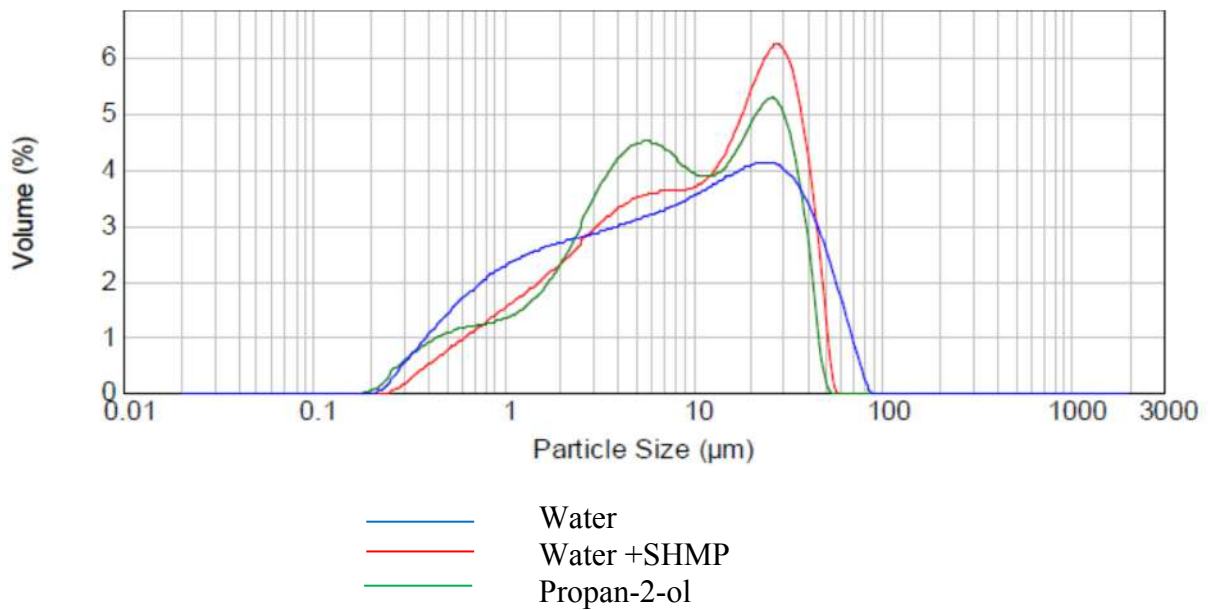
Figure 3. PSD frequency curves of GGBS (SSA=4700 cm 2 /g)
