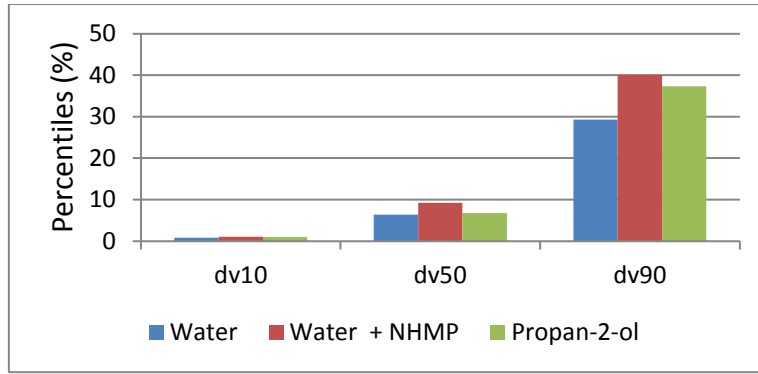
Figure 2. Volume weighted percentiles of GGBS (SSA = 5500 cm 2 /g)
