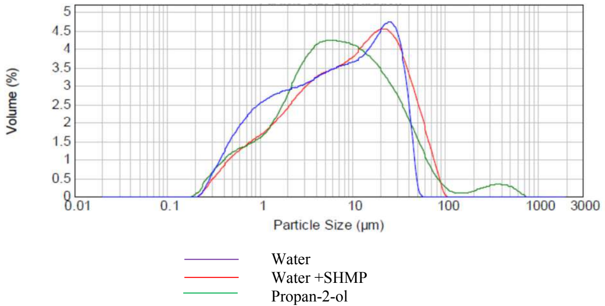
Figure 4. PSD frequency curves of GGBS (SSA=5500 cm 2 /g)
