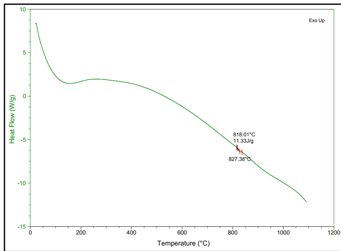
Figure 1. The DSC heating curve for the analyzed steel, highlighting the endothermic peak
