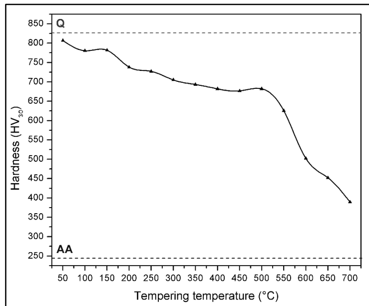
Figure 3. Change in hardness values after tempering quenched samples at different temperatures for 20 minutes; Q- after quenching; AA – after annealing
