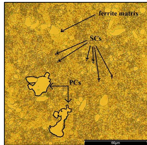
Figure 2. Investigated steel after annealing, magnification x1000
