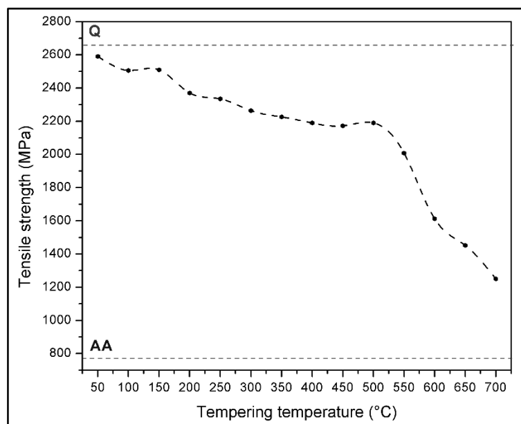
Figure 4. Change in tensile strength values calculated from the hardness values; Q- after quenching; AA – after annealing
