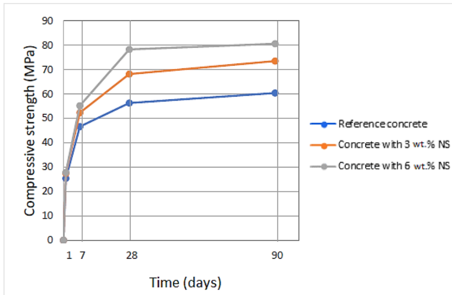
Figure 2. Concrete compressive strength development
