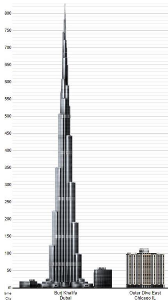
Figure 1. The Last Completed Super High–Rise, Burj Khalifa, 2010 (left) and the First Completed High- Strength Concrete High–Rise, Outer Drive East 1963 (right) [13]
