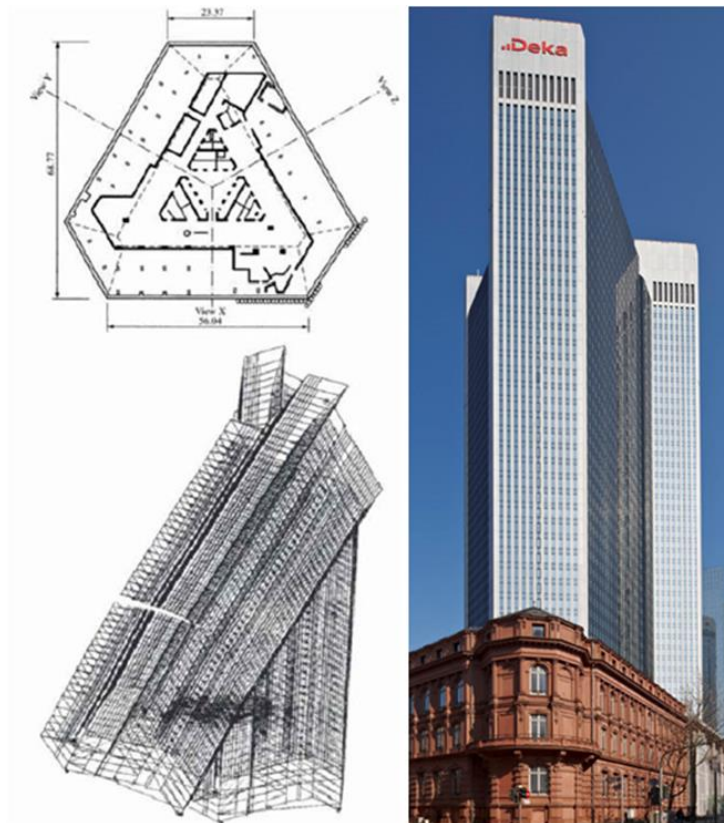
Figure 5. Characteristic Floor Plan of Trianon Building (left–top), Schematic Scenario of Possible Collapse (left–bottom) and Trianon Building, 1992, completed (right) [18,19]
