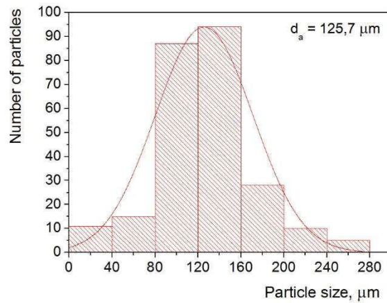
Figure 2. The average particle size ( d_a ) and particle size distribution of atomized copper powders (a) A-VF; (b) A-F; (c) A-M
