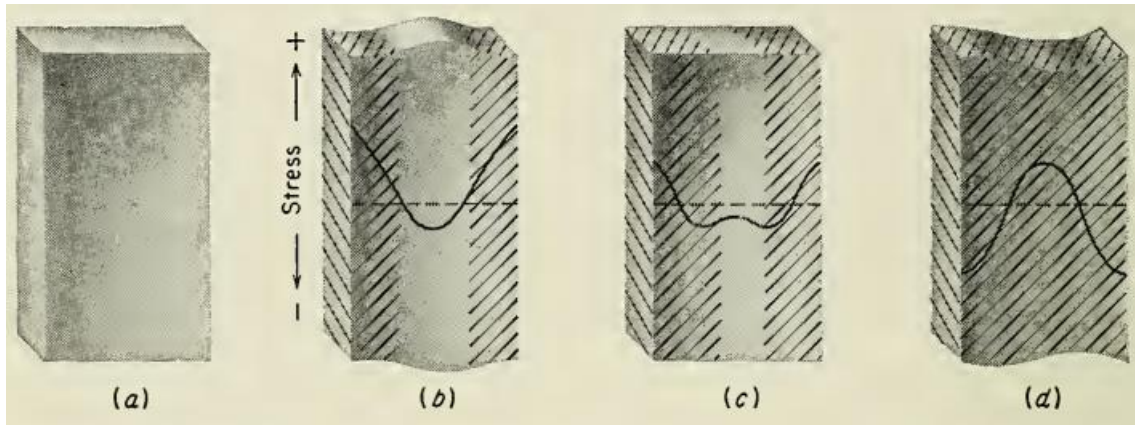
Figure 1. Development of residual stresses during cooling of a hot ingot. Cool portions shown shaded, [2]
