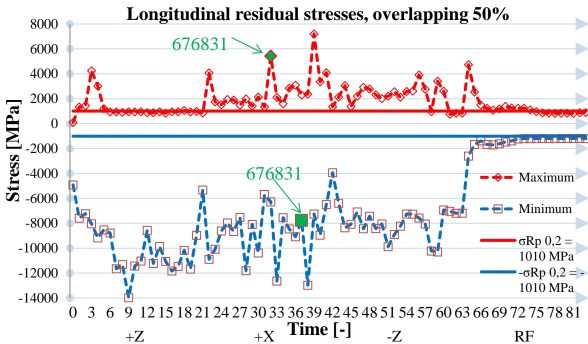
Figure 7. Investigation of “Bauschinger effect” in longitudinal direction with overlapping value of 50%
