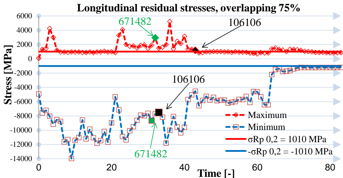
Figure 5. Investigation of “Bauschinger effect” in longitudinal direction with overlapping value of 75%
