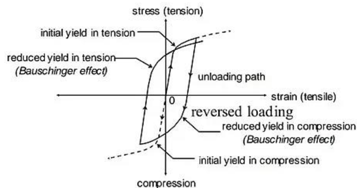
Figure 2. Schematic representation of Bauschinger effect [10]
