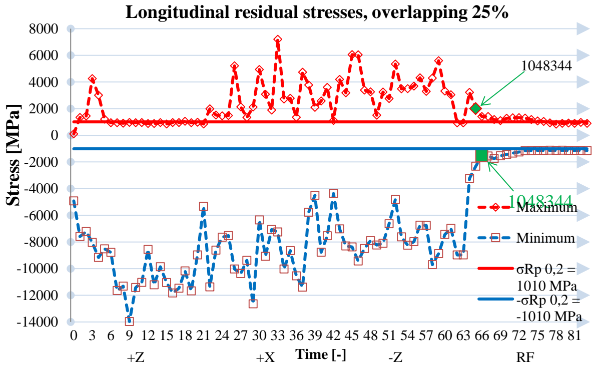
Figure 9. Investigation of "Bauschinger effect" in longitudinal direction with overlapping value of 25%
