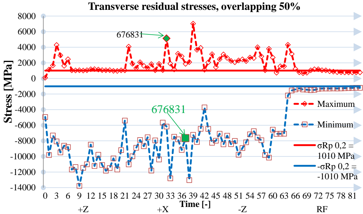
Figure 8. Investigation of "Bauschinger effect" in transverse direction with overlapping value of 50%
