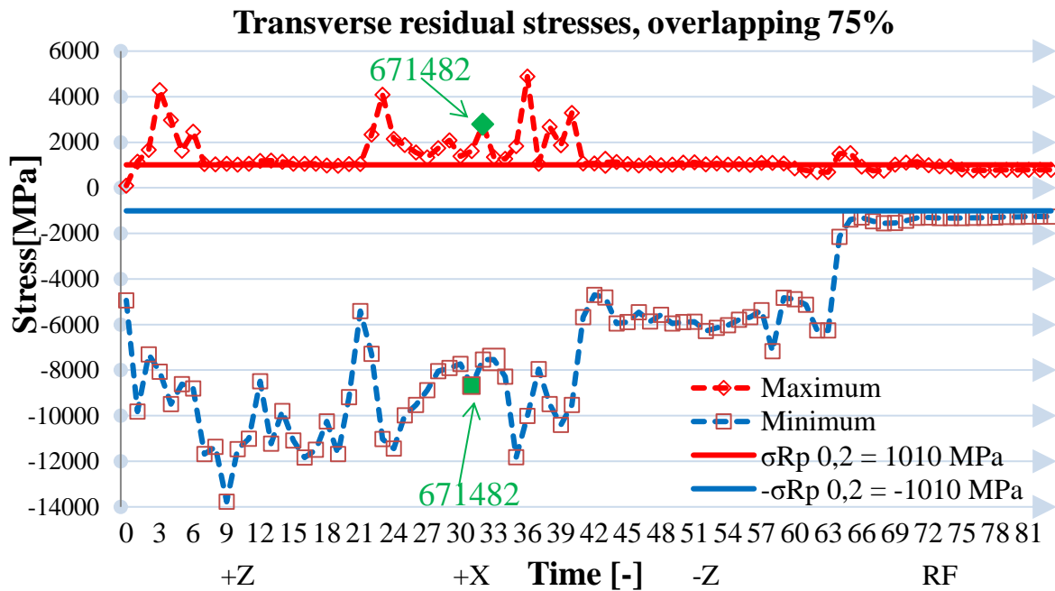
Figure 6. Investigation of “Bauschinger effect” in transverse direction with overlapping value of 75%
