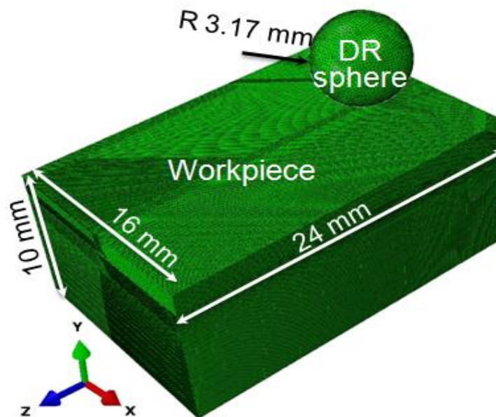
Figure 3. Assembly for the model [12]
