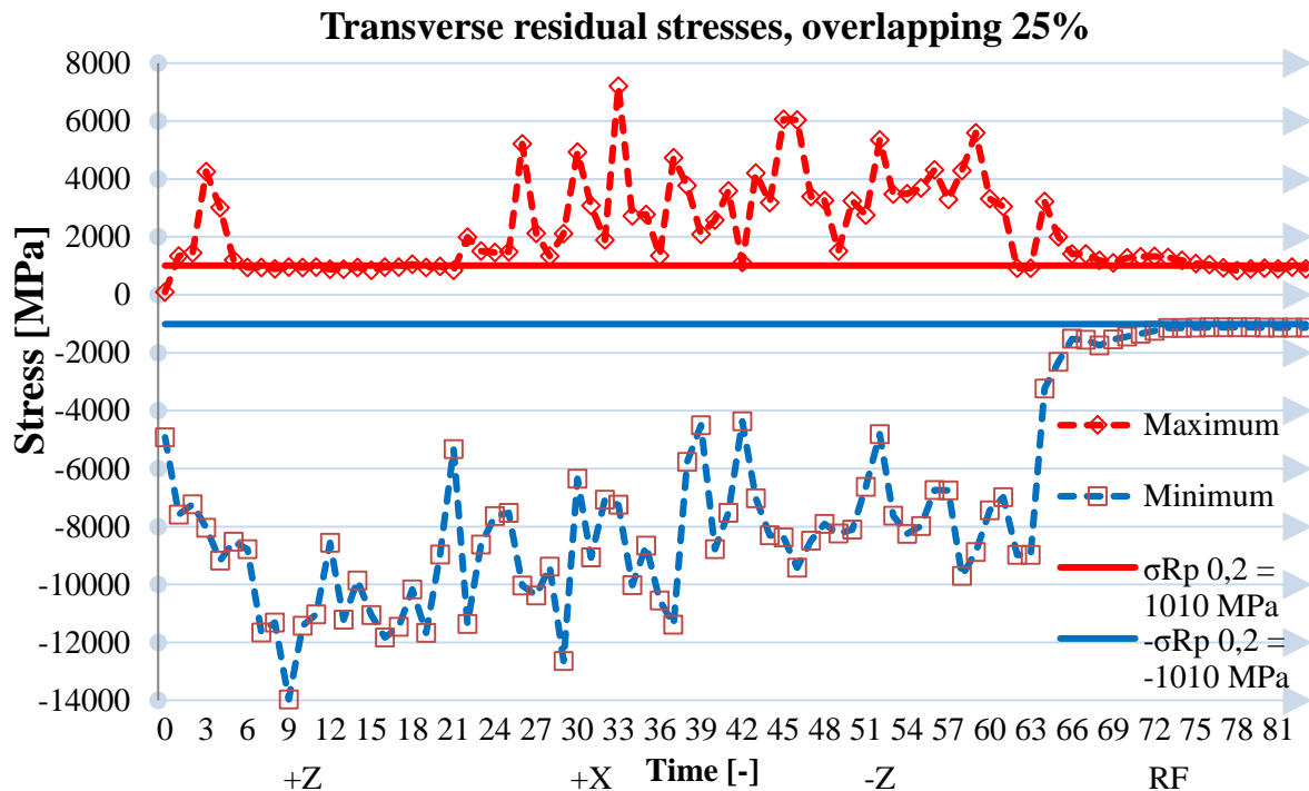
Figure 10. Investigation of “Bauschinger effect” in transverse direction with overlapping value of 25%
